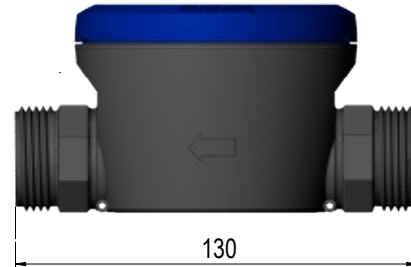
Type L – G1B x 130 mm
